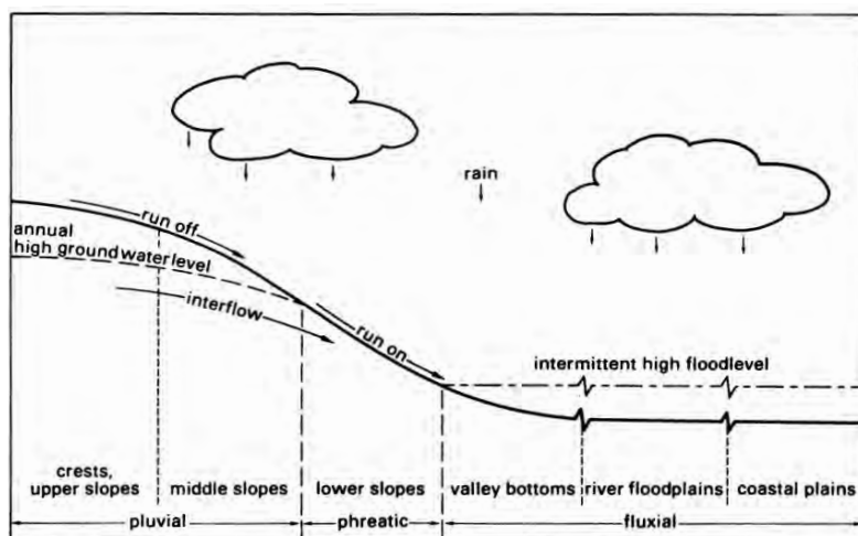
Figure 2.5 Landscape elements and physio-hydrography along a toposequence (from Andriesse and Fresco (1991)).
